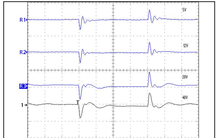
Figure 14: Output voltage response for 28V input; 5V, 12V, 28V, 40V output to step change in load current (50%-75%-50% of I_{out\ max} ; di/dt=0.1A/\mu s ). Load cap: 100uF electrolytic cap, V_{out} (2V/div); (500uS/div)
